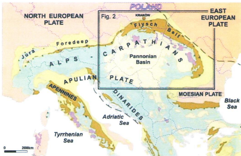
Fig. 1. Sketch of Alpine geology in Europe (after Picha, 1996; modified)
